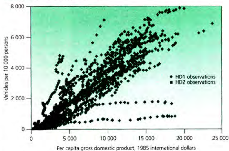
FIGURE 3.2 Motorization rate versus income*
