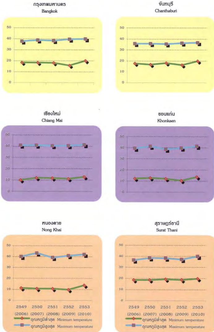
FIGURE 23.1 MAXIMUM AND MINIMUM TEMPERATURE AT SOME METEOROLOGICAL STATION: 2006 - 2010
