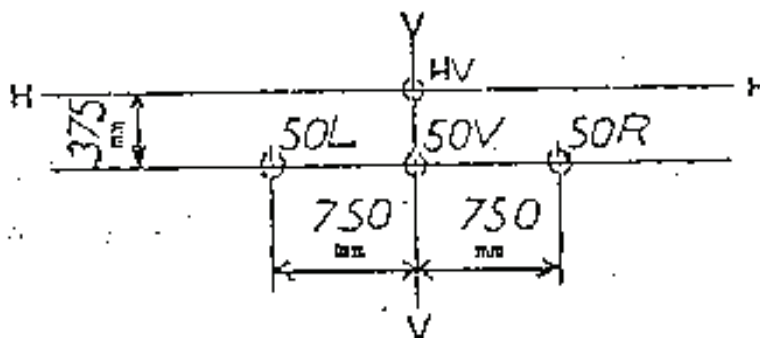
Diagram of Measuring Points on a Screen
